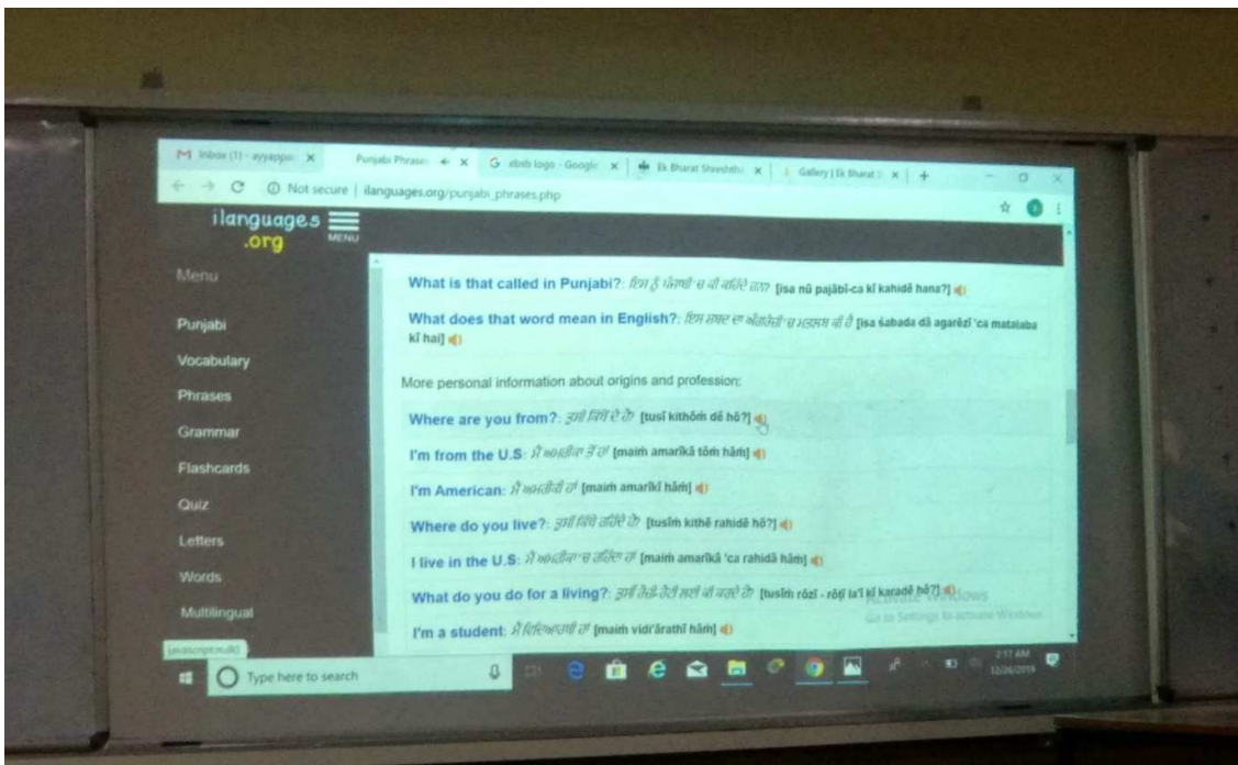
Punjabi sentences
