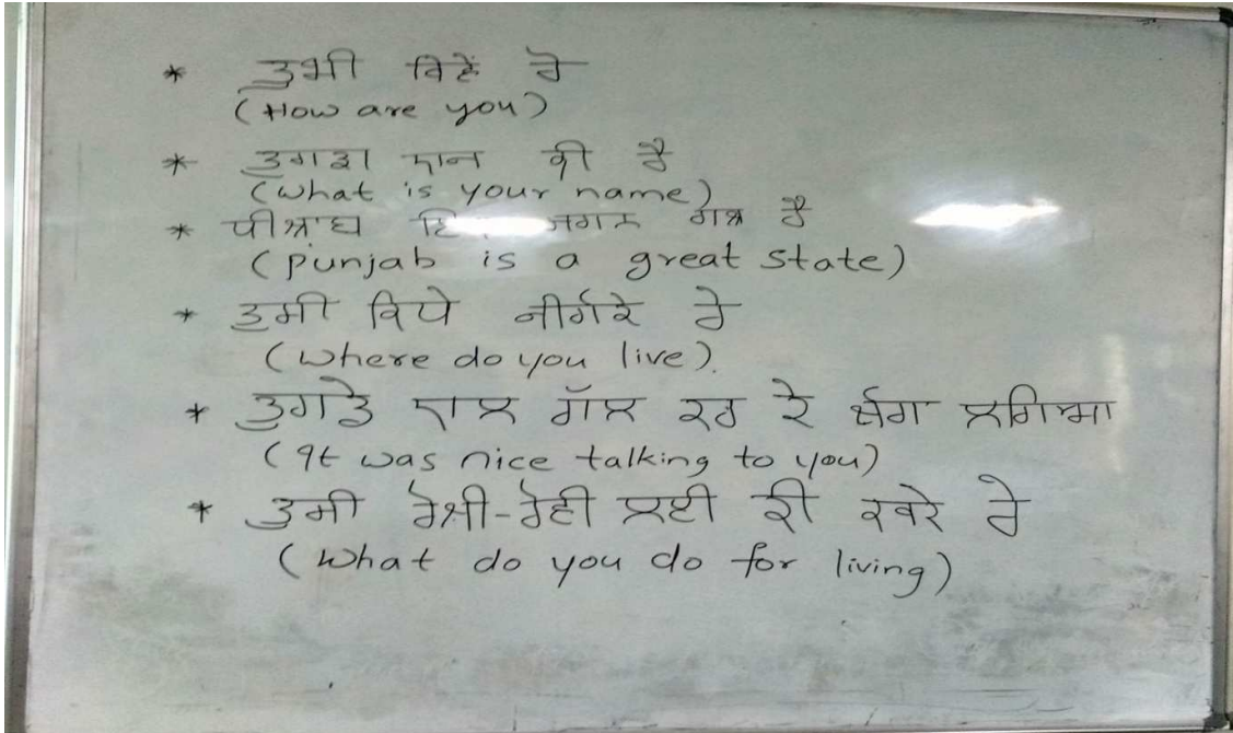
Punjabi sentences
